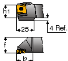
16mm shank configuration
